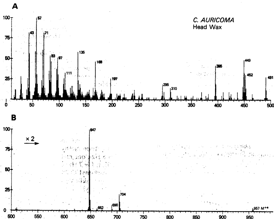
Fig. 1. Direct insertion probe mass spectrum of head wax from Cerogenes auricoma .
